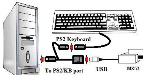
Typical Connection of the CBL-MXU-KB
